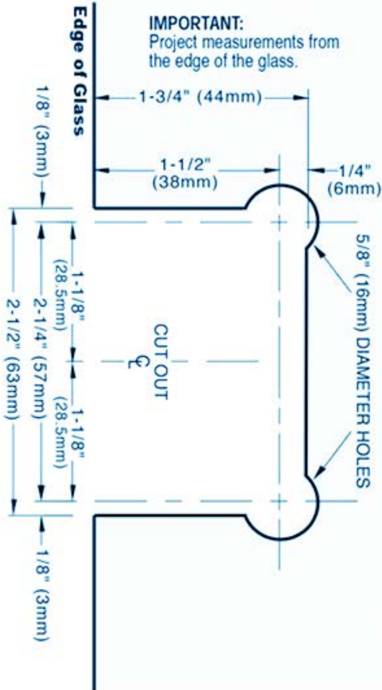
EMR92B Wall Mount Hinge
